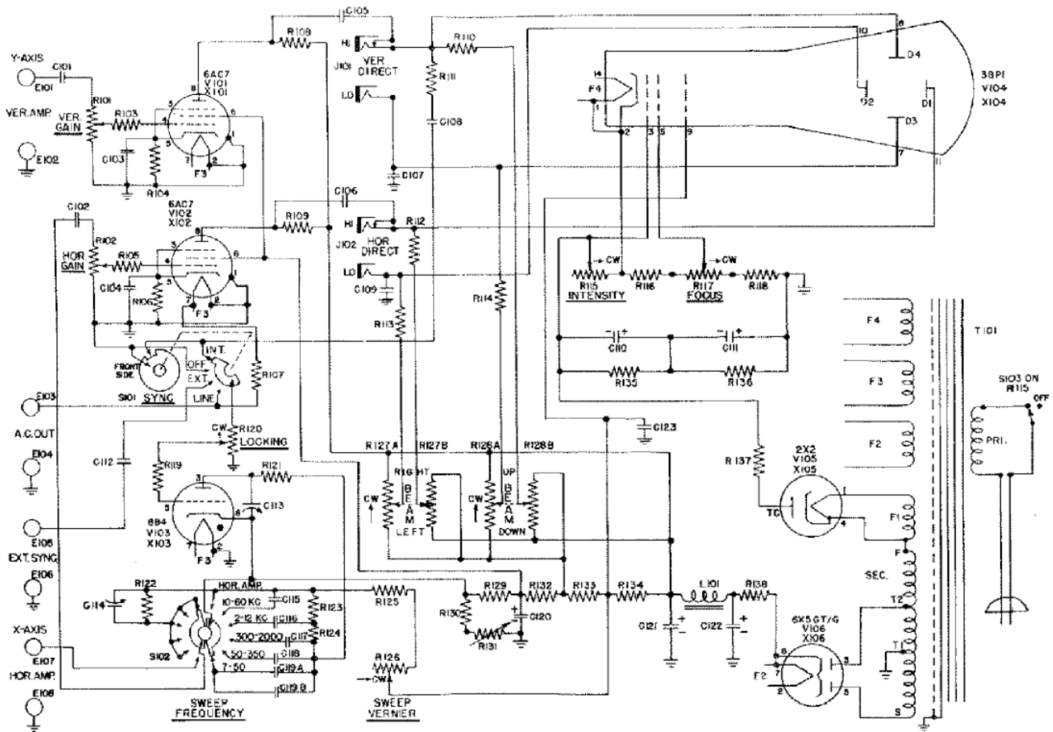
Schematic diagram of OBL-3 oscilloscope.
